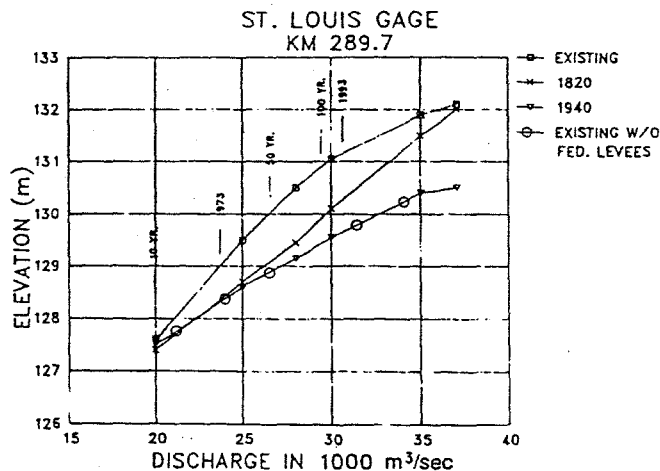
FIGURE 3 Stage discharge relationship at St. Louis Gage.
