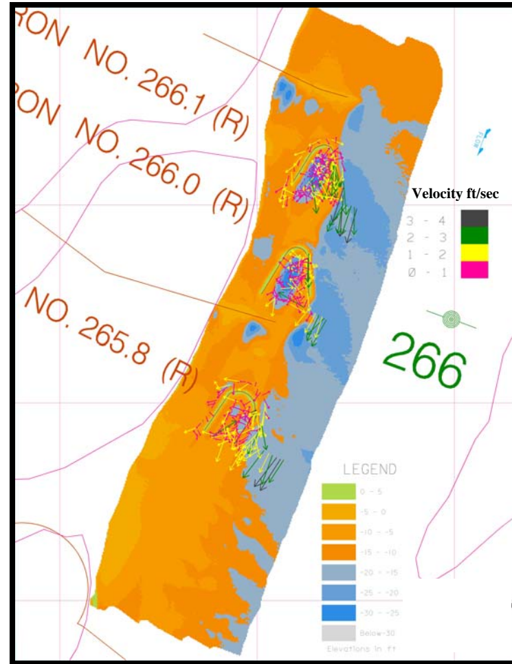
Figure 6. Velocity survey conducted at the Pool 25 chevron dikes in August and December 1999. Red arrows indicate flows suitable for over-wintering habitat (less than 1 ft per second). Note the higher flows (greens and grays) in the channel adjacent to the
