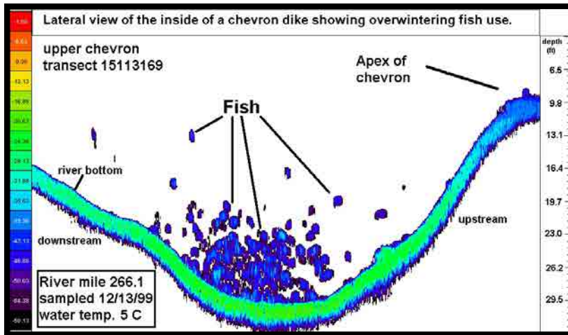
Figure 7. Hydroacoustic printout showing winter fish use of the upper chevron dike.
