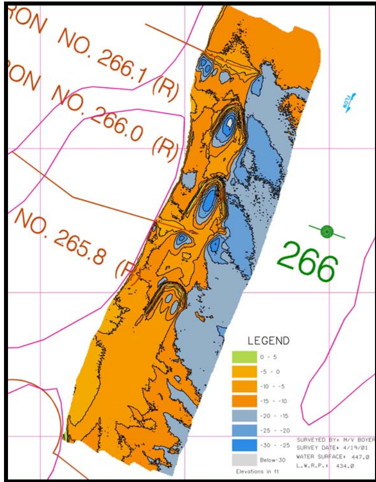
Figure 5. Bathymetric survey conducted at the Pool 25 chevron dikes in April 2001. The upper and middle chevron dikes show depths in excess of 25 ft. The depths behind the lower chevron dike are much shallower. Note the shorter riverside leg on the lower chevron dike.
