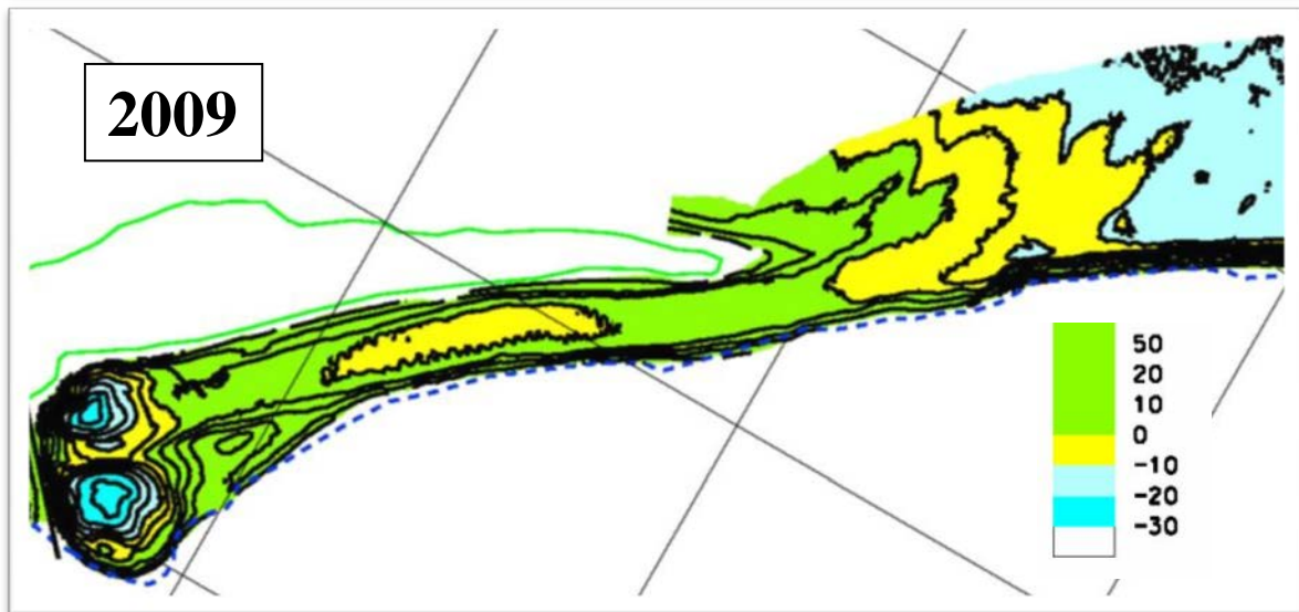
Post-dredging bathymetric surveys in the lower end of Sister Chute.
